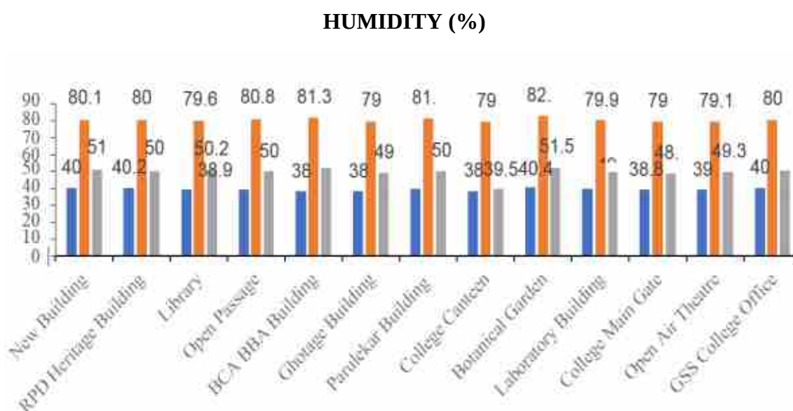
Graph no. 7.2 Humidity monitoring at college campus
